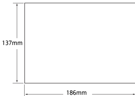
Panel Cut-out details. Allow 87mm depth.
